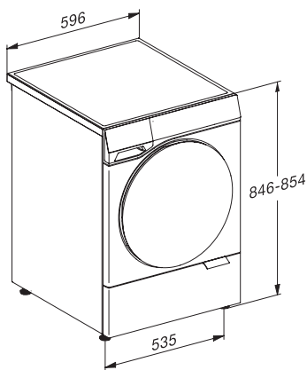
W2 drawing, facia 17 degree, Bigfoot, Ref2, measures in mm
