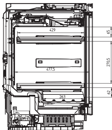
KWTUS7055F, interior dimensions (installation drawings)
